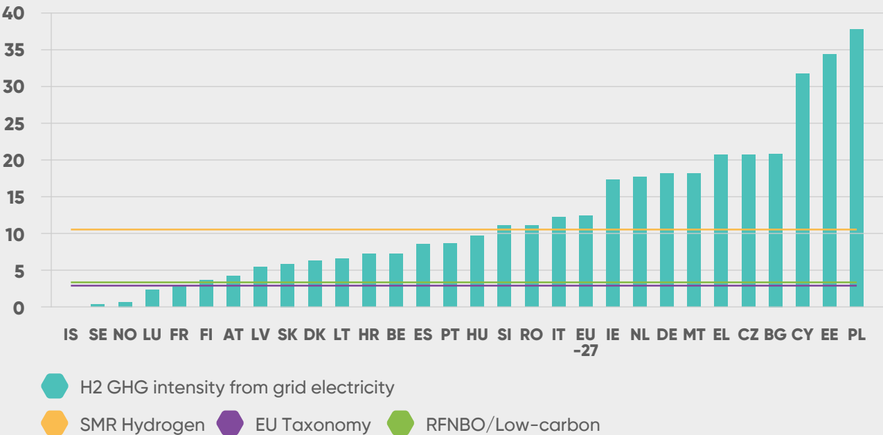
FIGURE 3.5 Carbon intensity of hydrogen produced from grid electricity, compared to selected benchmarks (tCO2/tH2)
